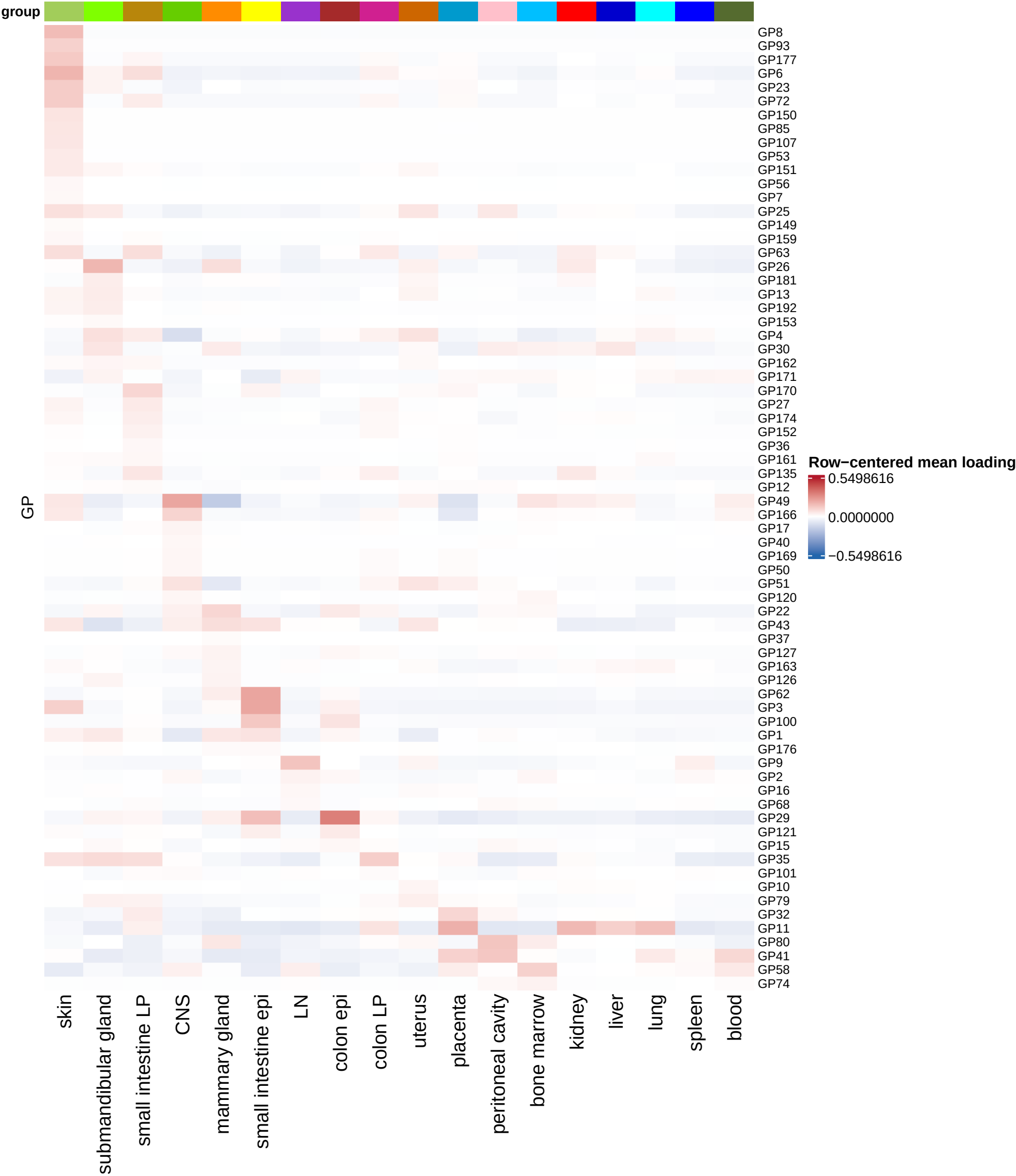
Row-centered GP mean loading: tissue (organ_simplified) dominant-group blocks (within block: dominance gap); focus: centered mean >= 0.01 filter
